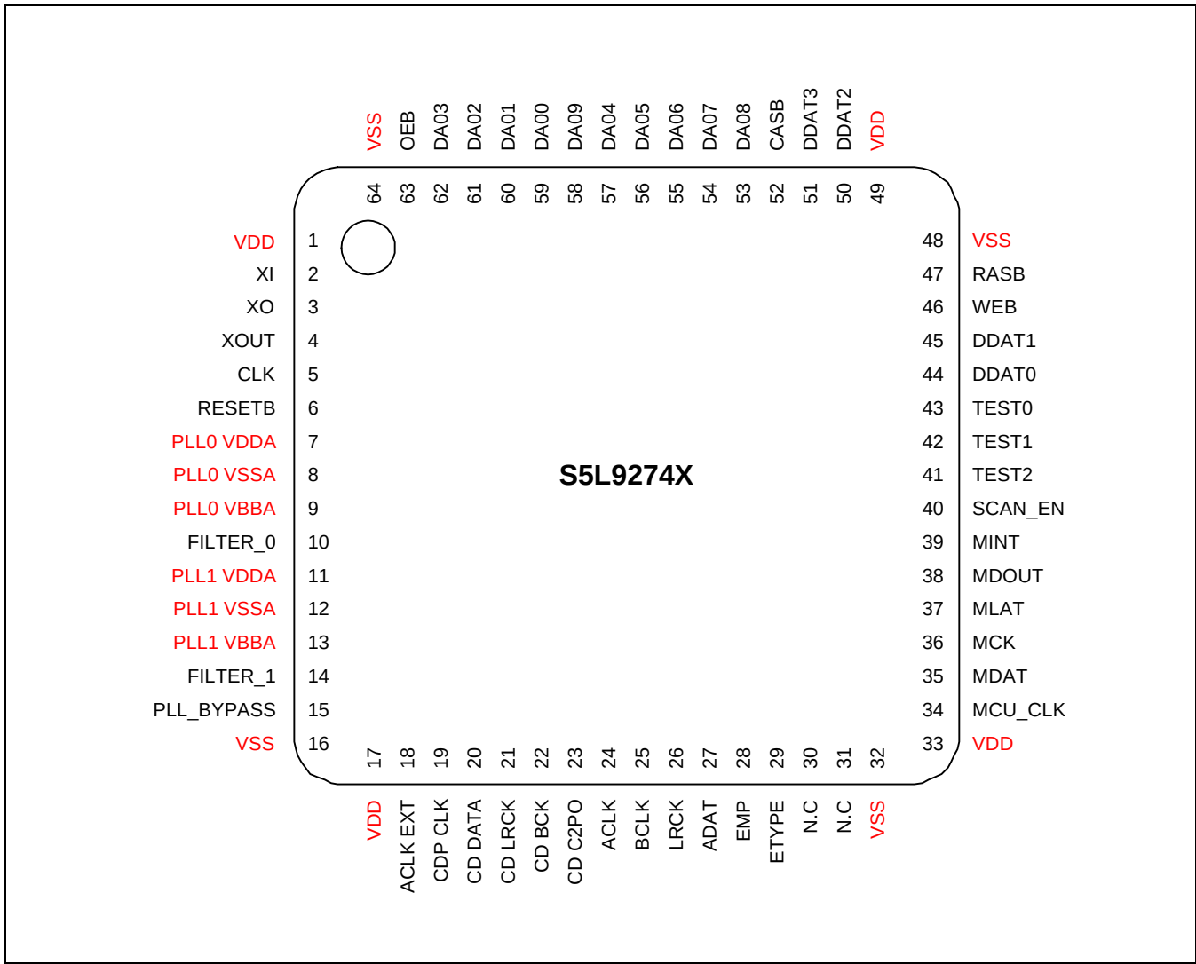
Figure 2. 64 pin Low profile Quad Flat Package (LQFP)
