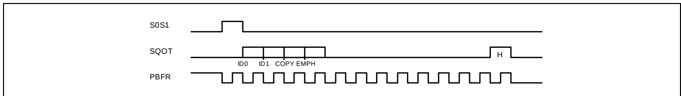
Figure 16. Timing Chart of Channel Status Data Output
