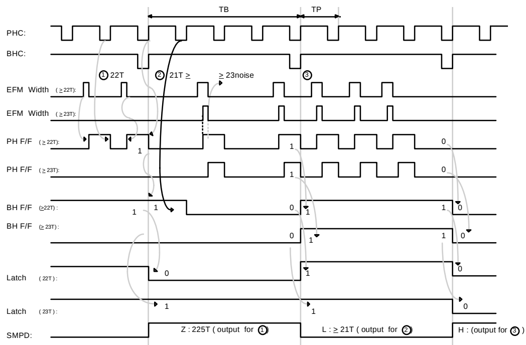
Figure 19. Timing Chart of SMPD Output When the Gain is "H" in the Speed Mode
