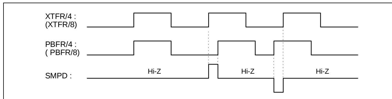
Figure 17. Timing Chart SMDP Output
