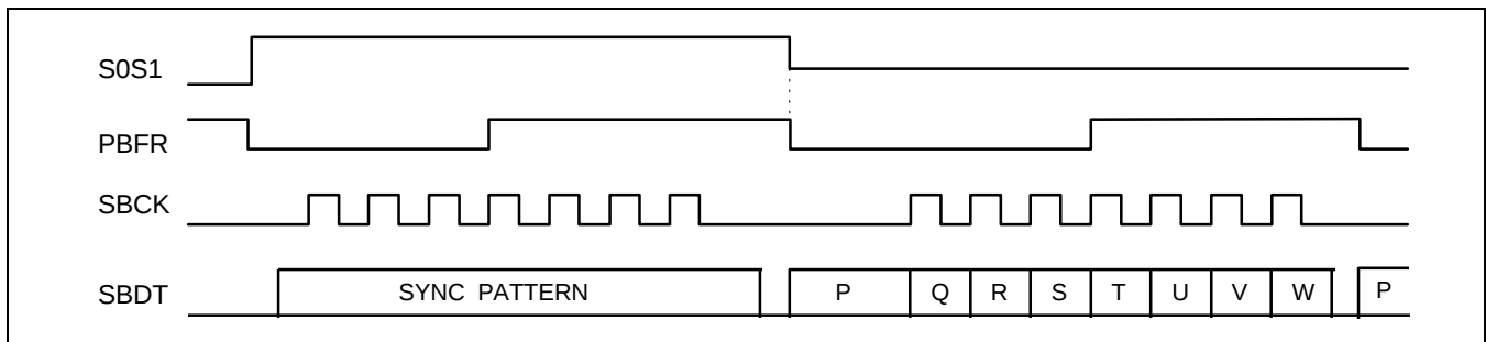
Figure 15. Timing Chart of Digital Audio Out
