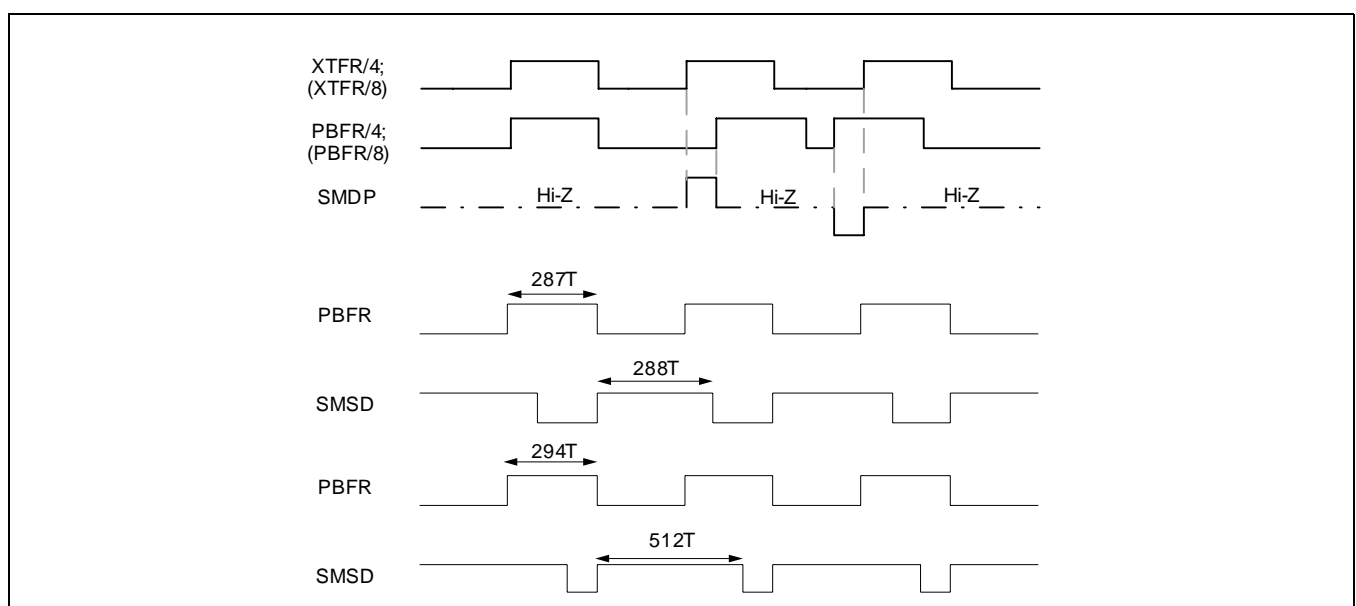
Figure 7. SMDP, SMSD Output Timing Diagram
