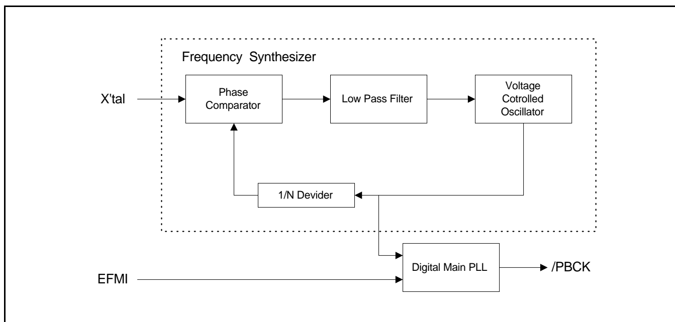
Figure 16. Digital PLL Circuit Diagram
