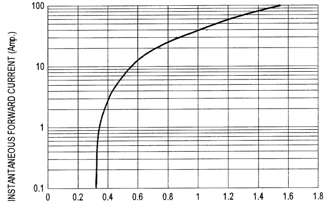
FIG-2 TYPICAL FORWARD CHARACTERISTICS
