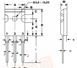
TO-247 (3P)
