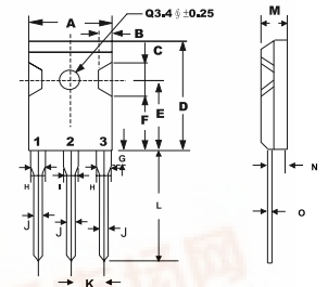
TO-247 (3P)
