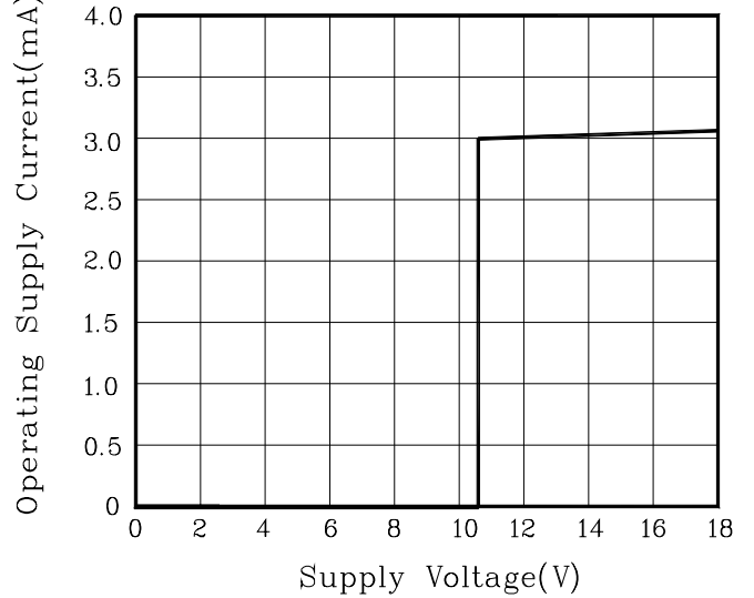
Fig. 6 Maximum Supply Voltage vs. Supply Current
