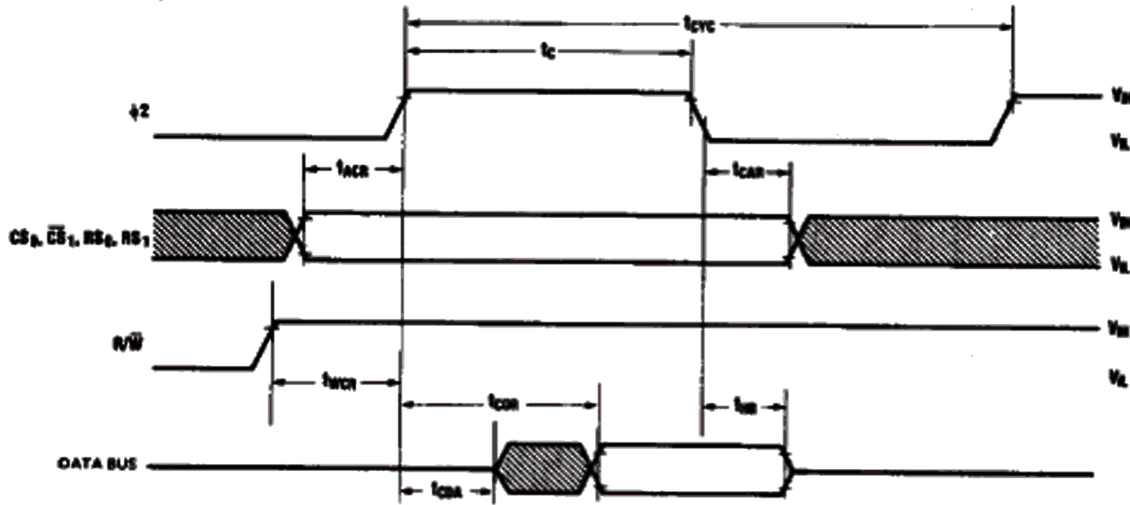
Figure 4. Read Timing Characteristics
