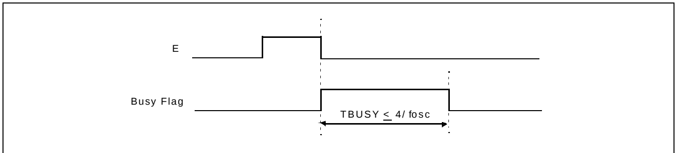
Figure 1. Busy Timing
