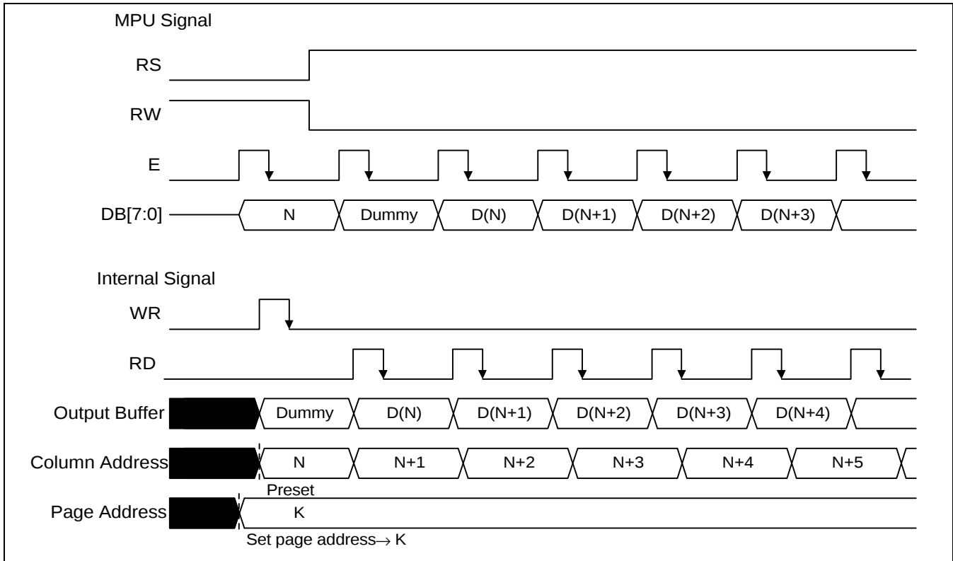
Figure 4. Read Timing
