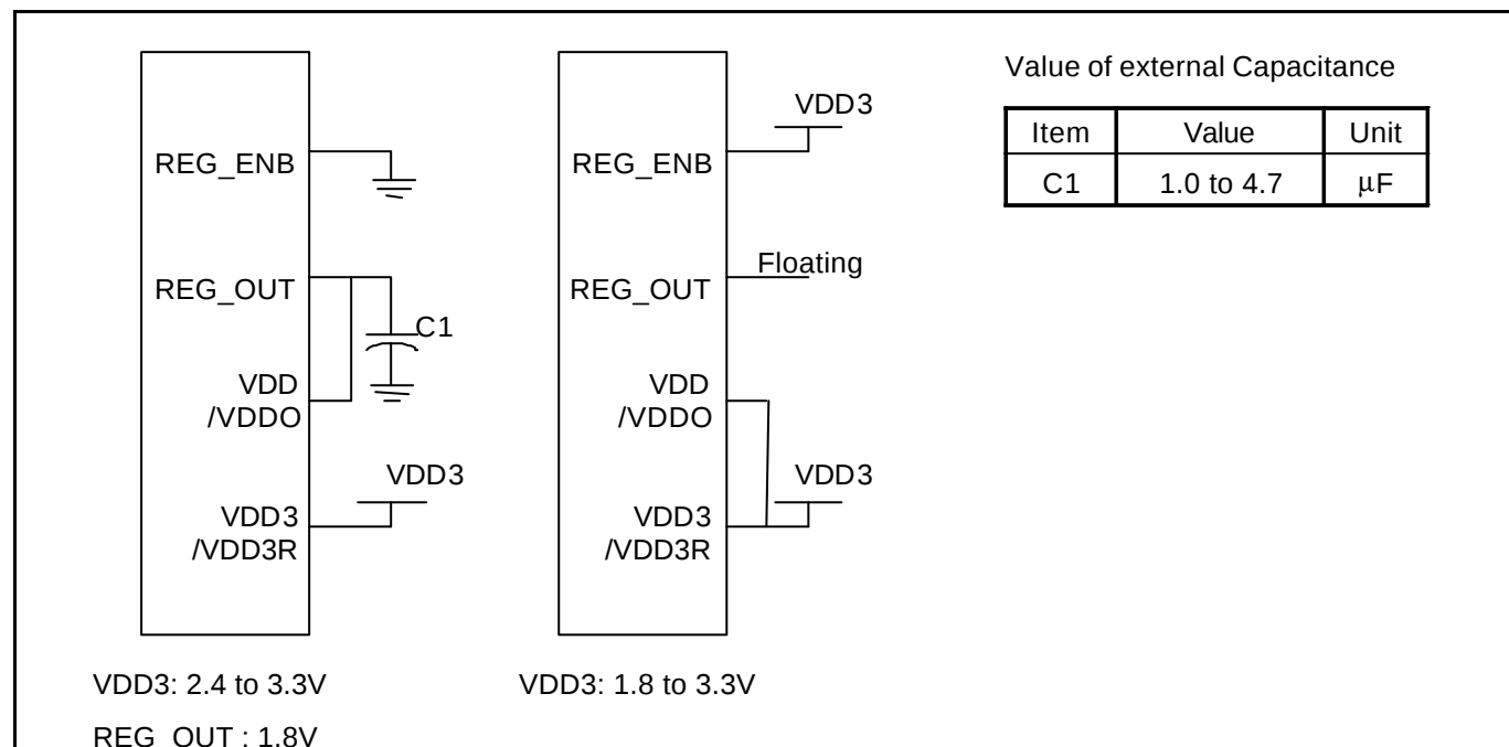
Figure 20. Regulator Application
