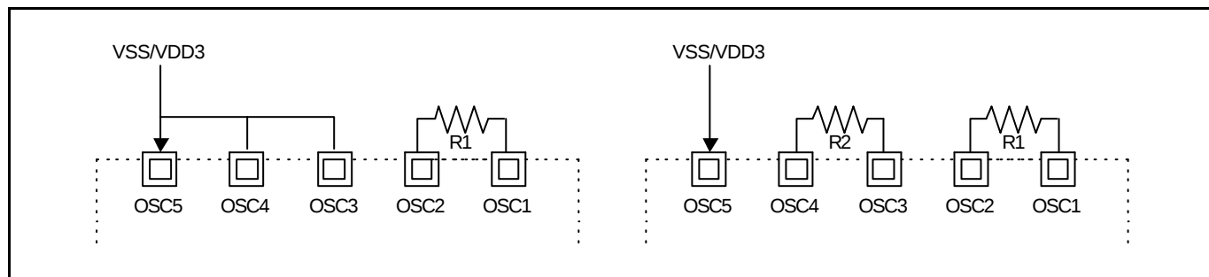
Figure 22. Internal oscillator application
