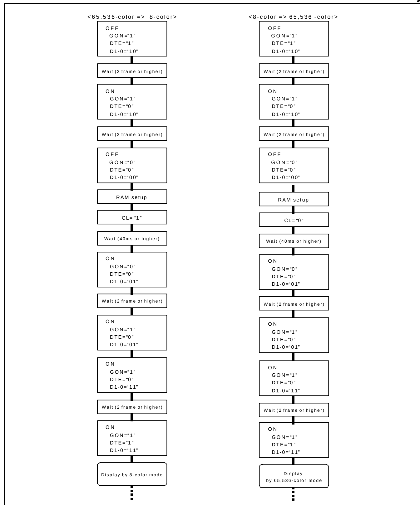
Figure 43. Set up procedure for the 8-color mode
