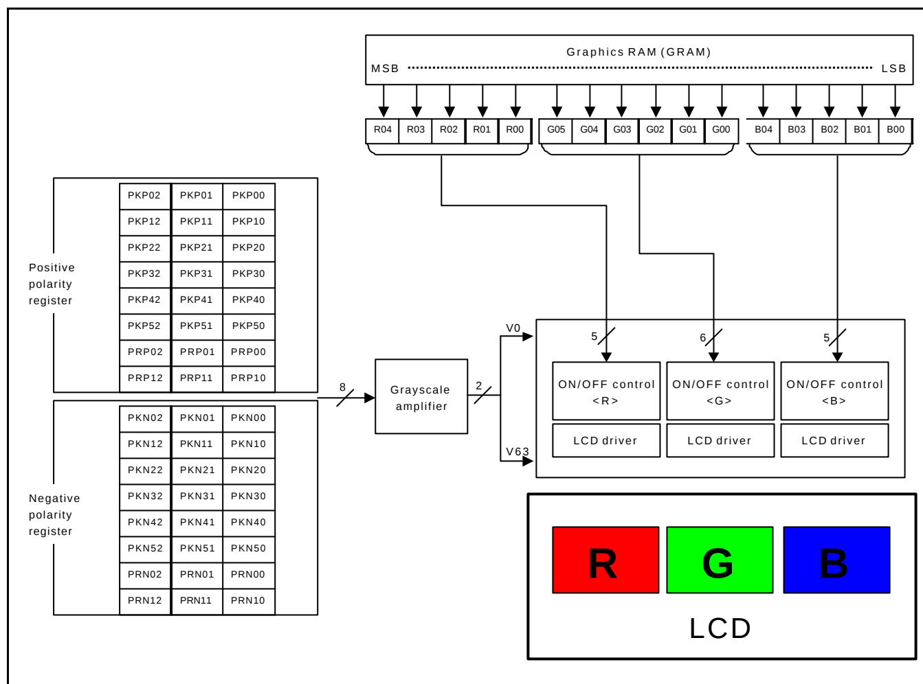
Figure 42. 8-color display control
