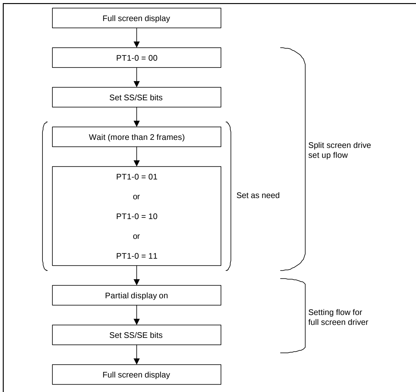
Figure 53. Partial display set up flow
