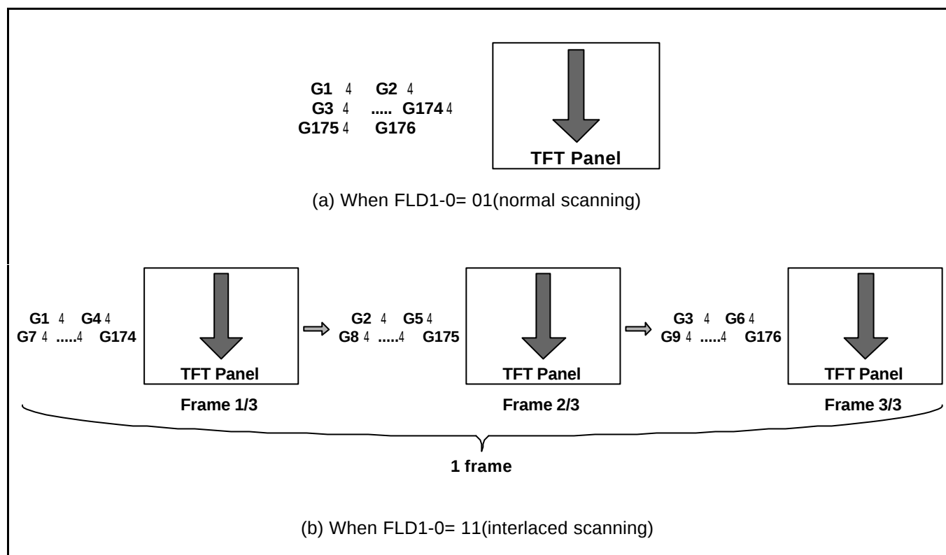
Figure 8. n raster-row interlaced scanning method
