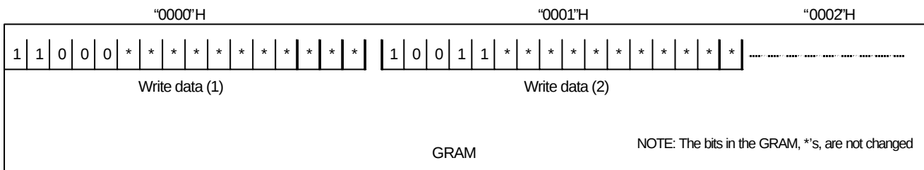
Figure 27. Writing operation of write mode 1
