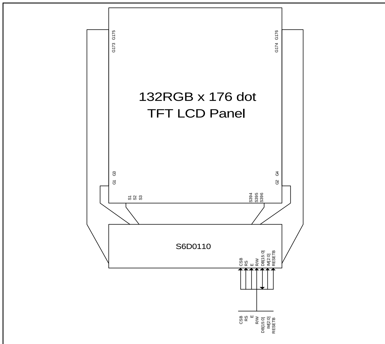
Figure 44. System structure
