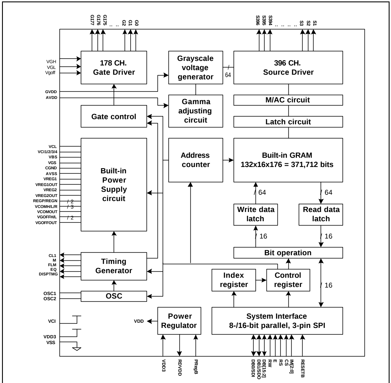
Figure 1. Block Diagram
