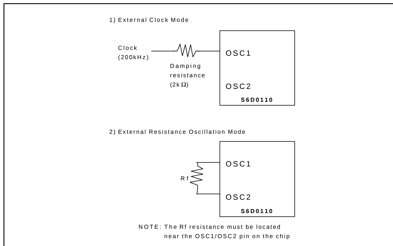
Figure 47. Oscillation Circuit
