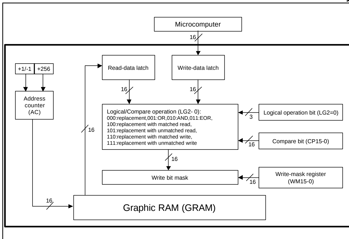
Figure 25. Data processing flow of graphic operation
