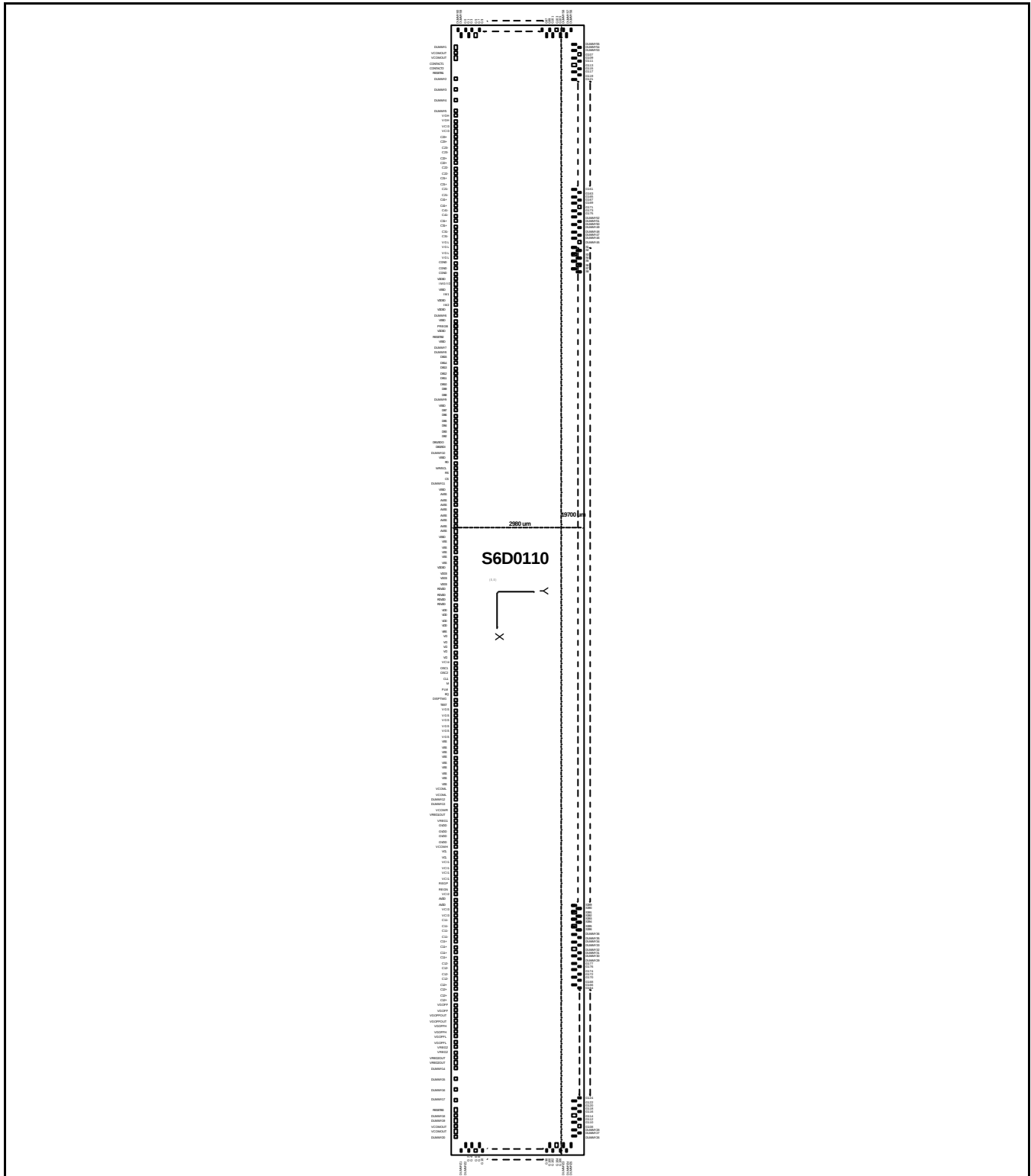
Figure 2. Pad Configuration
