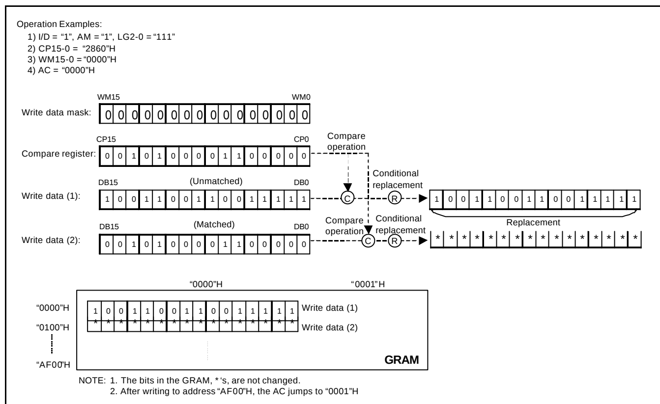
Figure 30. Writing operation of write mode 4
