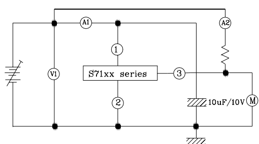
Test Circuit 1
