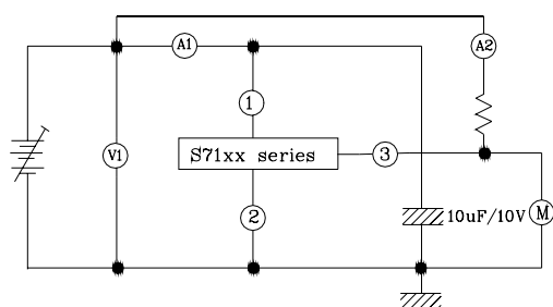
Test Circuit 1
