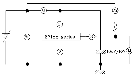
Test Circuit 1
