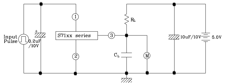
Test Circuit 2
