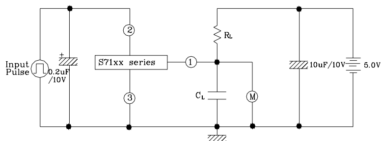
Test Circuit 2
