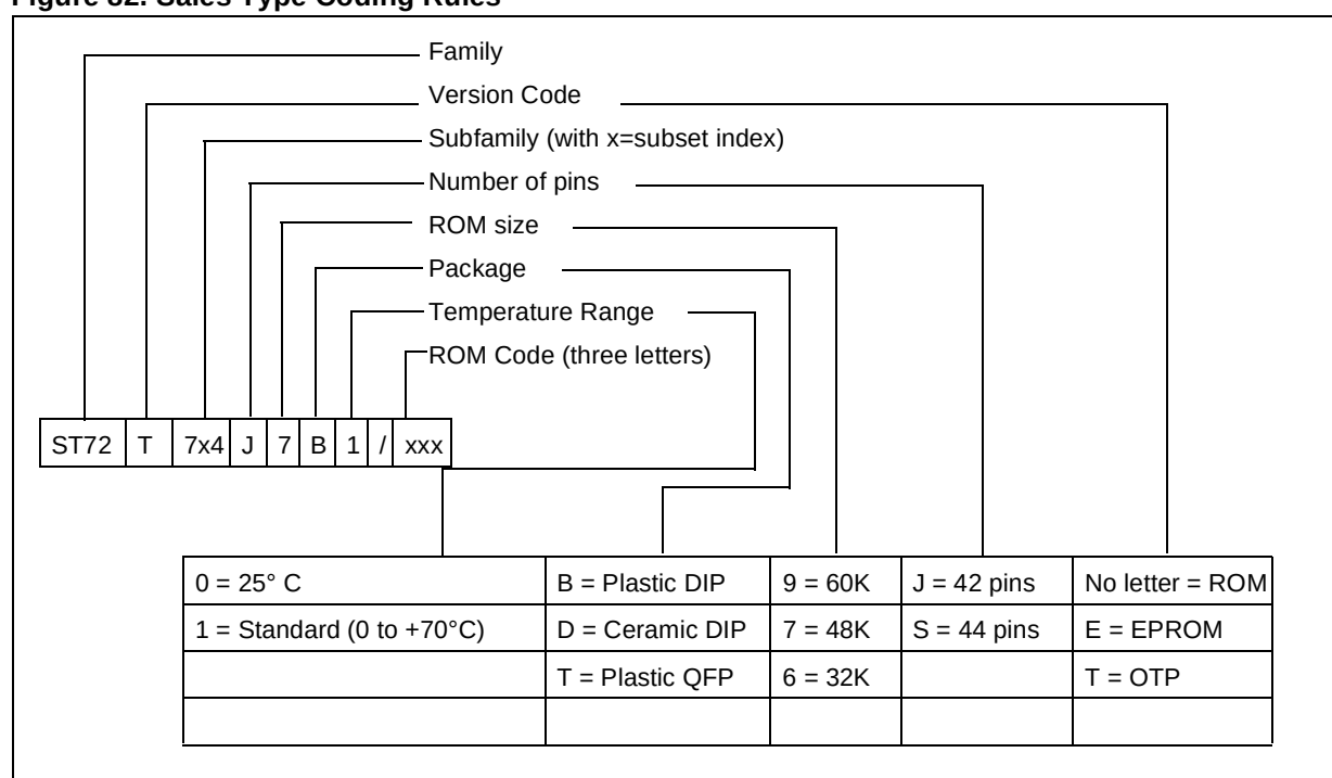
Figure 82. Sales Type Coding Rules
