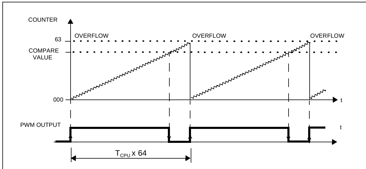
Figure 69. PWM Generation
