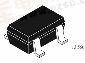
S822TW Marking: W22 Plastic case (SOT 343) 1 = Collector, 2 = Emitter, 3 = Base, 4 = Emitter
