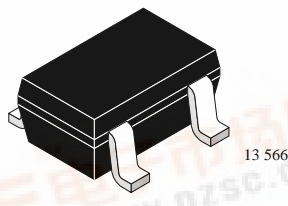
S822TRW Marking: WSF Plastic case (SOT 343R) 1 = Collector, 2 = Emitter, 3 = Base, 4 = Emitter
