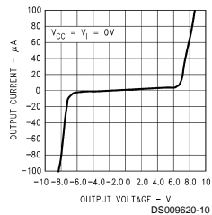
Output Current vs Output Voltage (Power Off)
