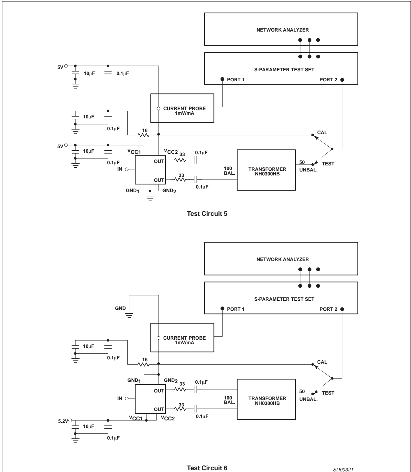
Figure 4. Test Circuits 5 and 6
