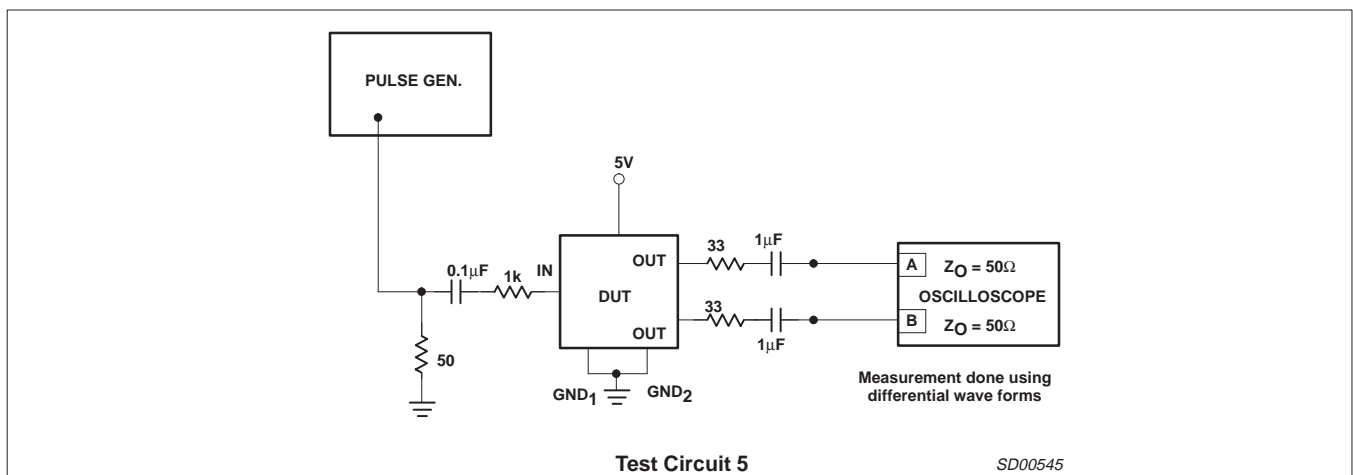
Figure 5. Test Circuit 5
