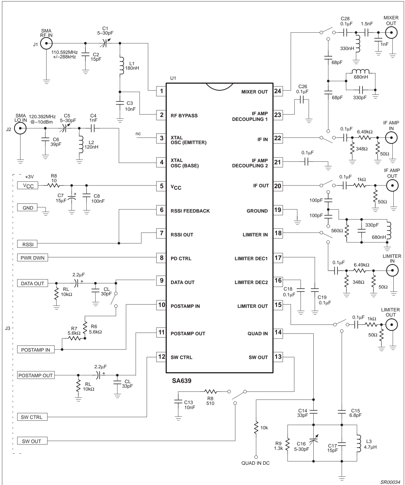
Figure 5. SA639 Test Circuit
