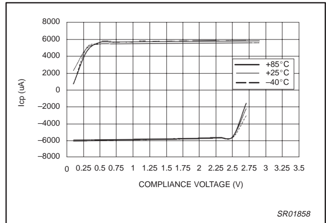
Figure 12. PHI Charge Pump Output vs. Temperature (CP = 00; V DD = 3.0 V; I SET = 165.33 μA)
