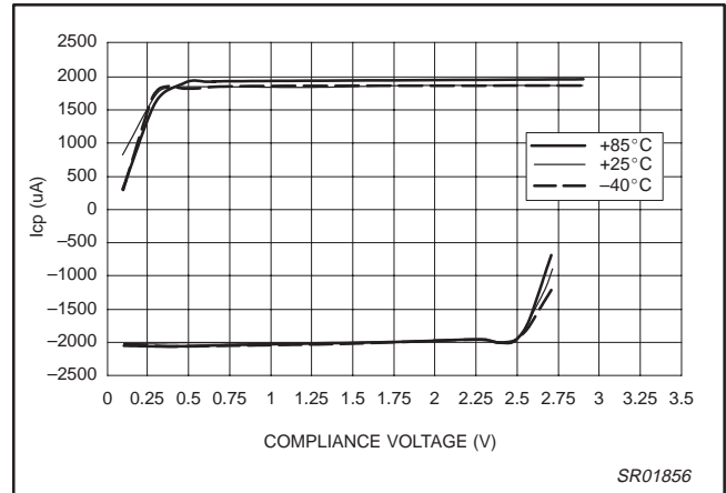
Figure 10. PHI Charge Pump Output vs. Temperature (CP = 01; V DD = 3.0 V; I SET = 165.33 μA)
