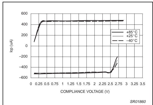
Figure 14. PHP Charge Pump Output vs. Temperature (CP = 10; V DD = 3.0 V; I SET = 165.33 μA)
