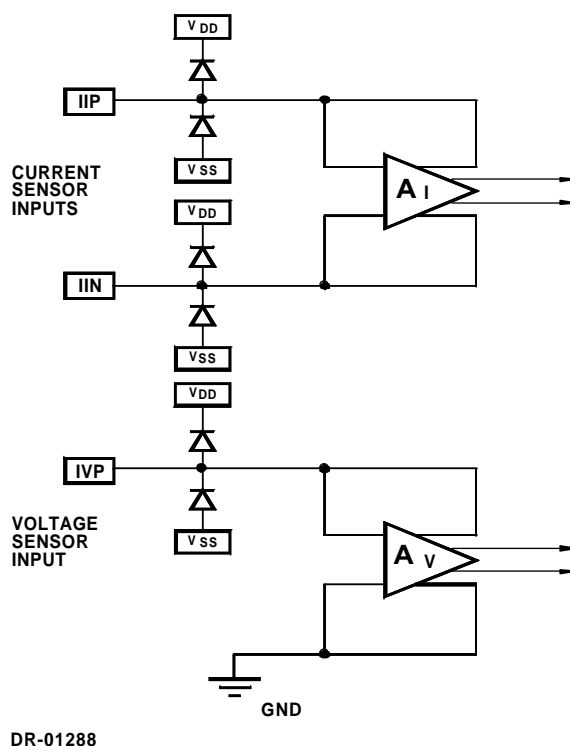
Figure 3: Analog Input Internal Configuration
