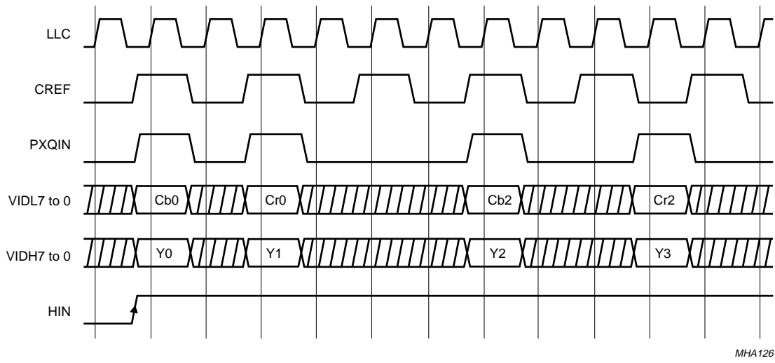
Fig.6 Timing of PXQIN for 16-bit data input from DMSD to expansion port.
