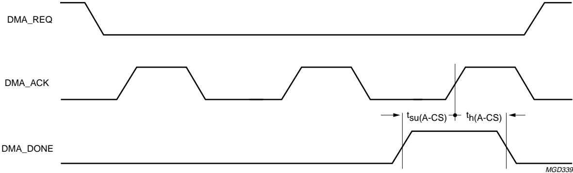
Fig.19 DMA_DONE timing.
