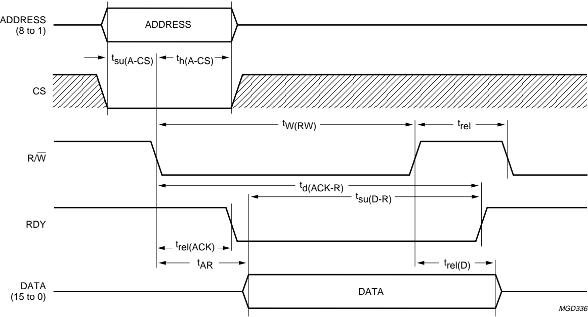
Fig.16 Intel read timing (non-multiplexed).
