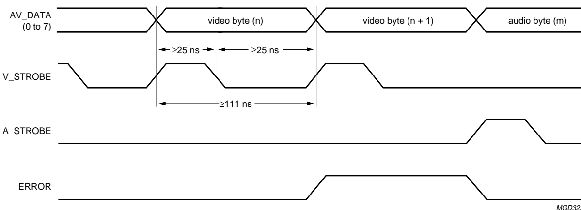
Fig.3 Timing diagram of parallel input mode.
