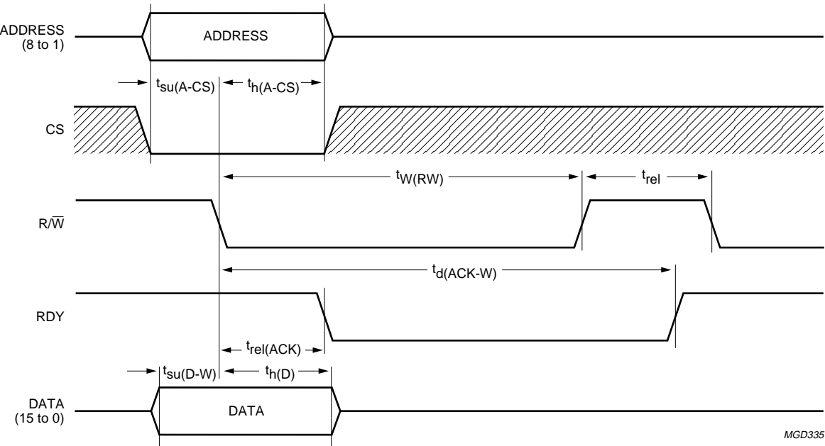
Fig.15 Intel write timing (non-multiplexed).
