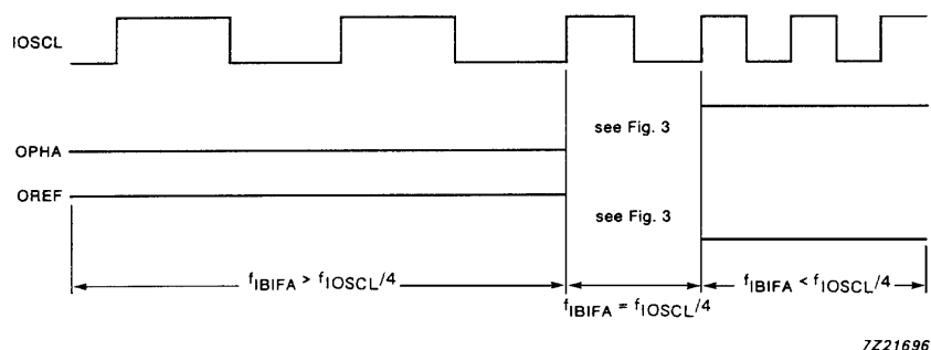
Fig.4 Generation of phase output signal (OPHA) and phase reference signal (OREF); f_{IBIFA} = f_{IOSCL}/4 .
