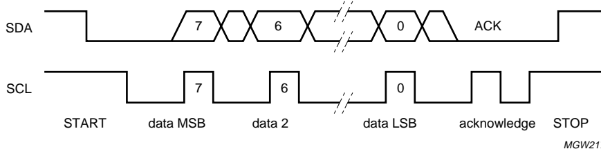
Fig.34 I 2 C-bus interface data transfer sequence.
