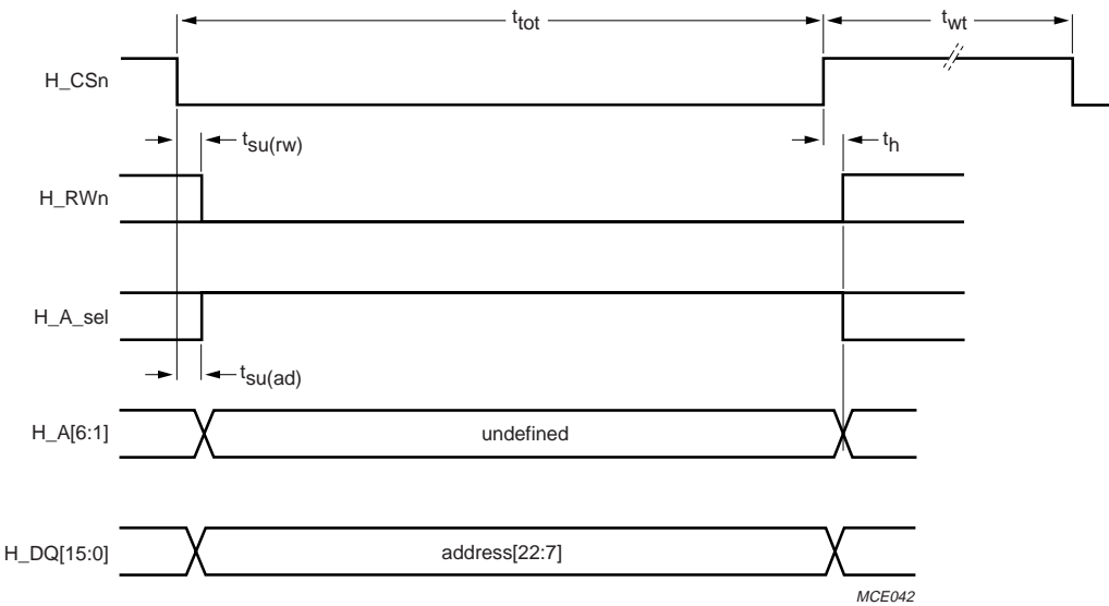
Fig 17. Timing diagram of writing the base address.
