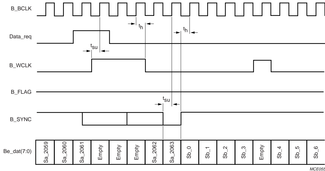
Fig 39. Timing diagram for UDE interface with sync edged triggered mode.
