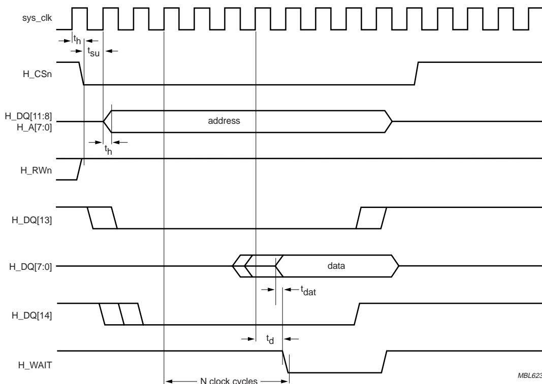
Fig 32. Timing diagram SAD08 read from the SAA7893HL.
