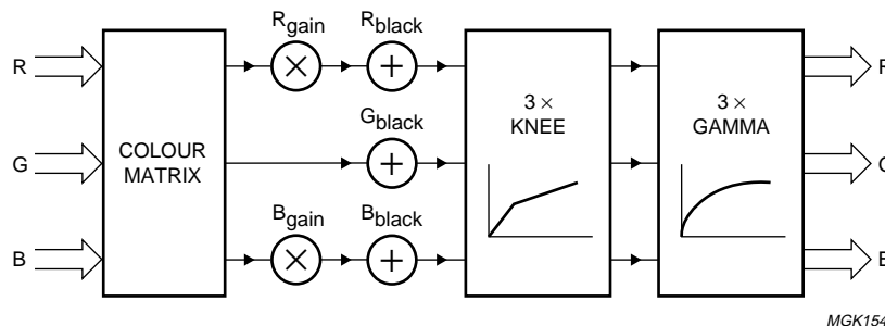
Fig.4 RGB processing.
