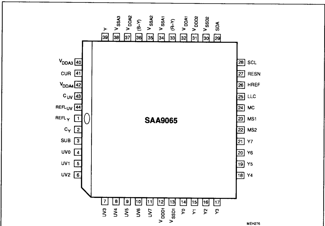
Fig.2 Pin configuration.
