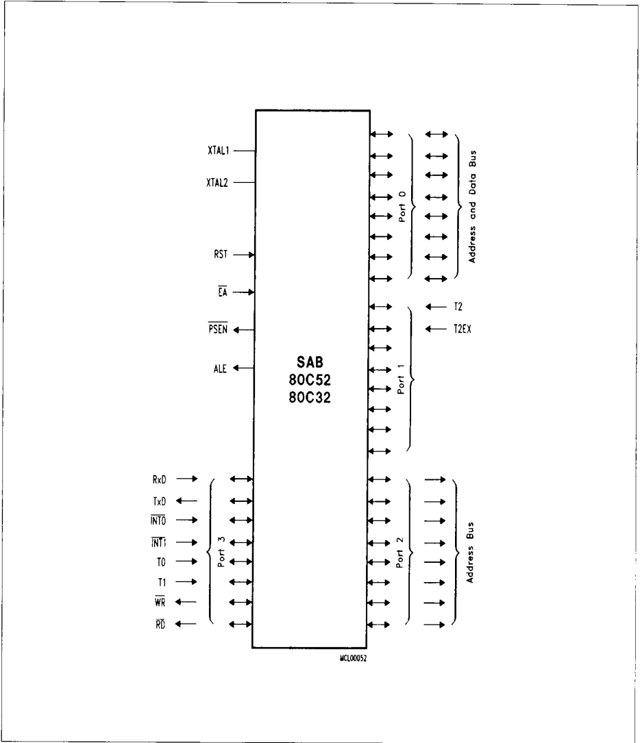
Logic Symbol
