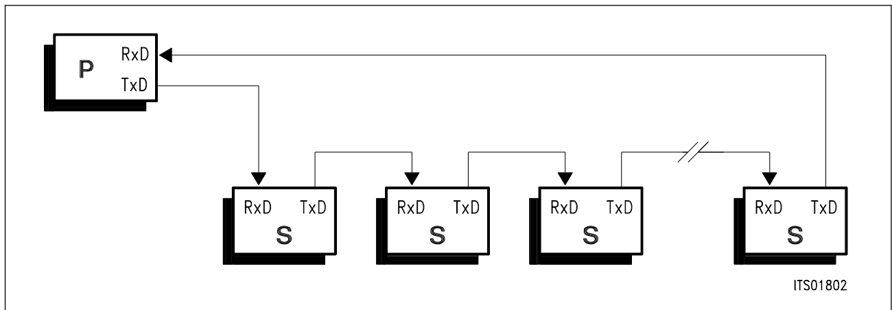
Figure 31 SDLC Loop
