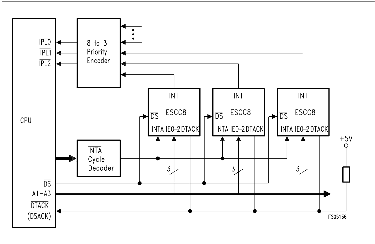
Figure 8 Interrupt Cascading (Slave Mode) in Motorola Bus Mode
