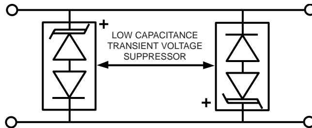
FIG. 4 - AC LINE PROTECTION APPLICATION
