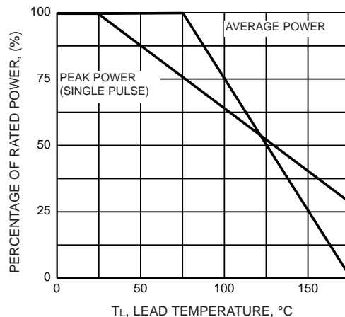
FIG. 2 - POWER DERATING CURVE
