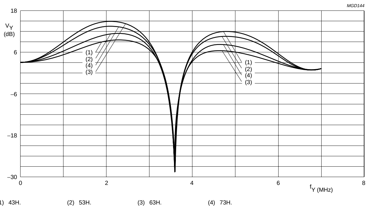
Fig.16 Luminance control SA 09H, 3.58 MHz trap/CVBS mode, prefilter on, different aperture band-pass centre frequencies.
