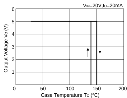
Thermal Protection Characteristics (SAI01)
