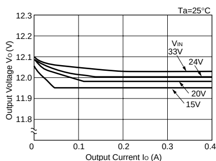
Load Regulation (SAI03)
