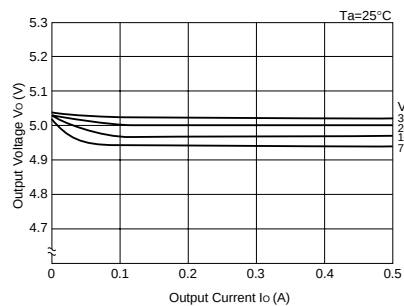
Load Regulation (SAI01)
