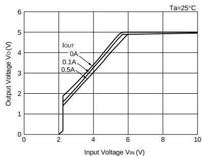
Rise Characteristics (SAI01)
