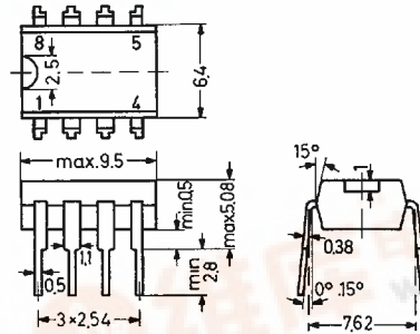
Fig. 1: SAK215 in mini Dip plastic package similar to TO-116 20A8 according to DIN 41866
