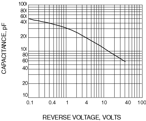
Fig. 5-TYPICAL JUNCTION CAPACITANCE
