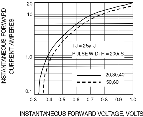
Fig. 4-TYPICAL FORWARD CHARACTERISTICS
