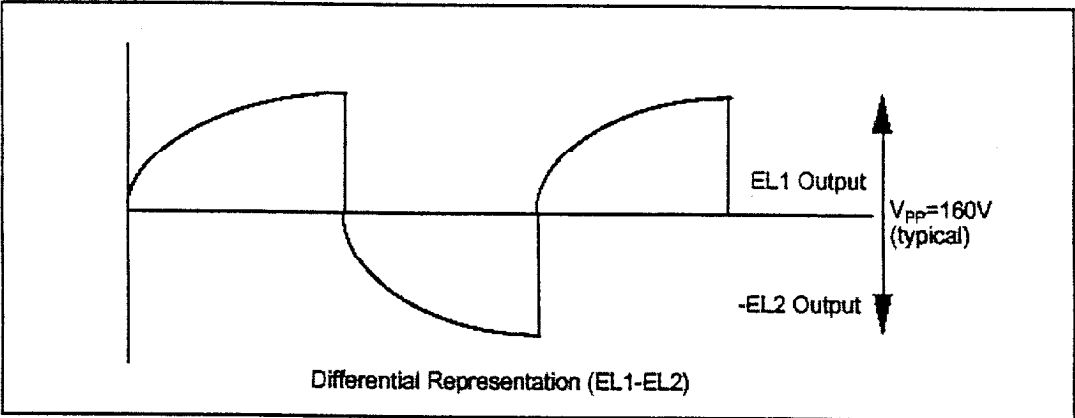
Figure 4. EL differential representation (EL1-EL2)
