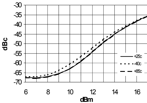
Adj. Channel Pwr. vs. Channel Output Pwr.
