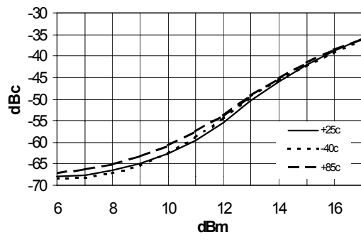
Adj. Channel Pwr. vs. Channel Output Power
