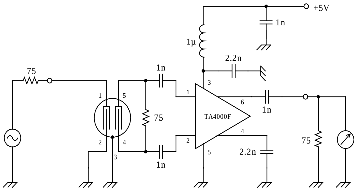
Fig.2 Evaluation circuit
