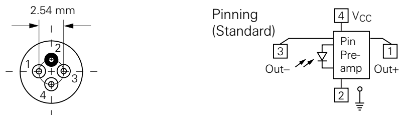
Figure 2 Receiver with Preamp
