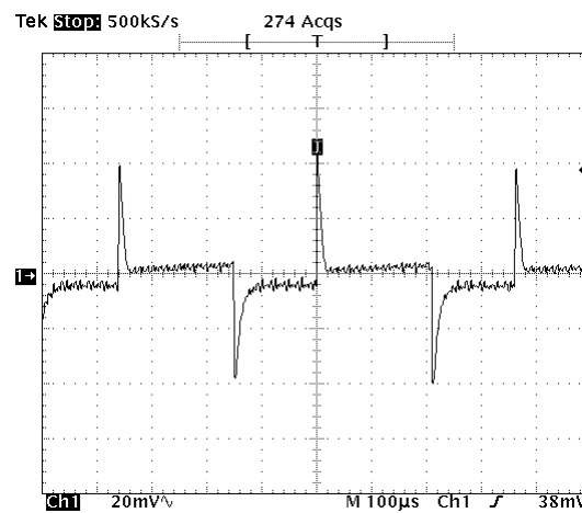
Transient Voltage Response 1.8V From 0.2 to 10A
