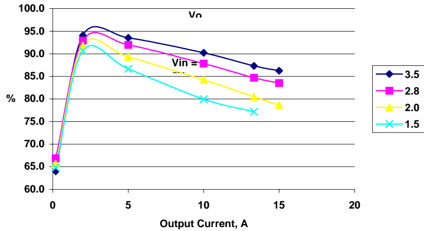
SC1154 Efficiency
