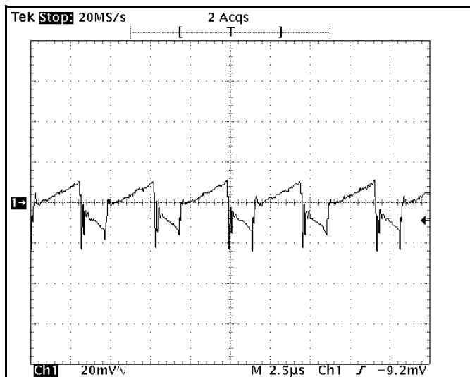
Typical Ripple, Vo=2.8V, Io=10A
