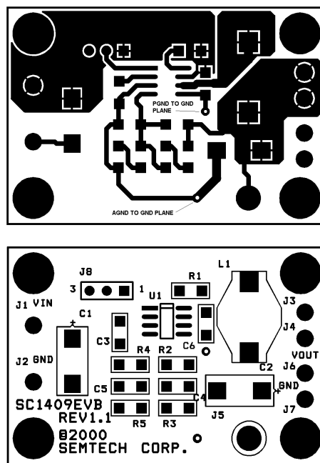
Evaluation Board Top Copper and Assembly Diagrams
