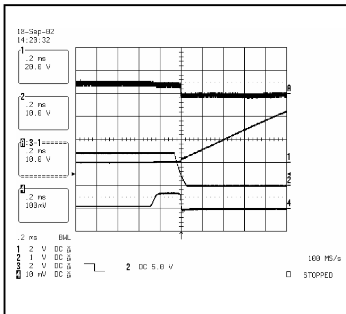
Figure 10. Over-current/Short circuit.
