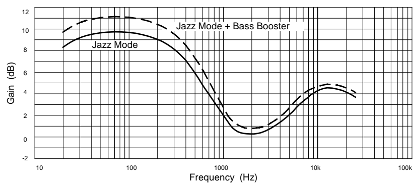
Fig.5 Jazz Mode(Jazz mode + Bass Booster)
