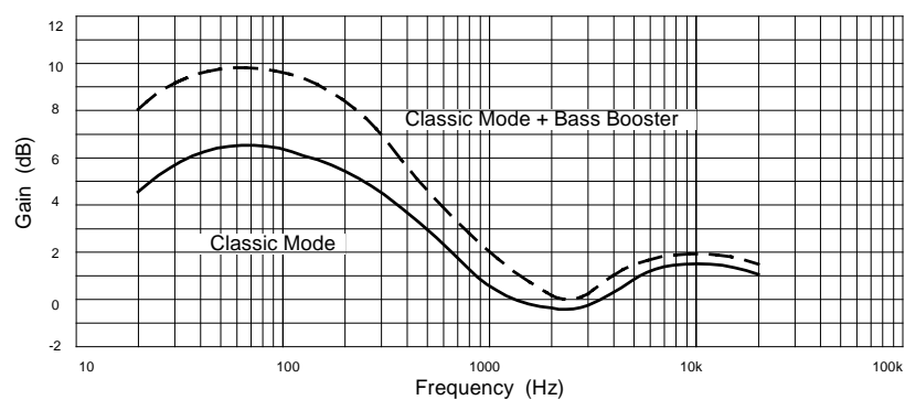
Fig.4 Classic mode(Classic mode + Bass Booster)
