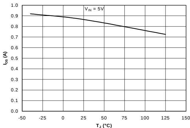
Short Circuit Output Current vs. Junction Temperature
