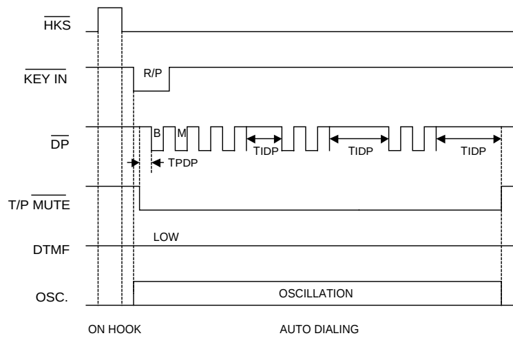
Figure 1(b). Pulse Mode Timing Diagram
