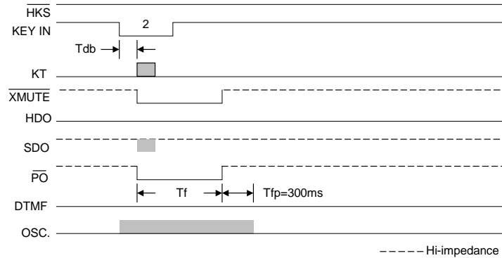
Flash key operating timing
