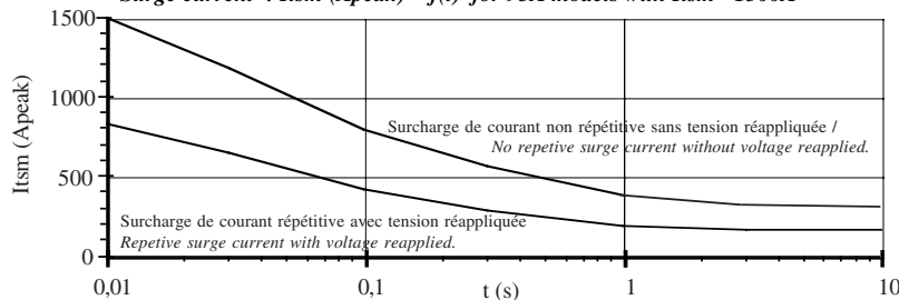
Fig.3 Surchage de courant : Itsm (Apeak) = f(t) pour modèle 95A(Itsm=1500A) Surge current : Itsm (Apeak) = f(t) for 95A models with Itsm =1500A
